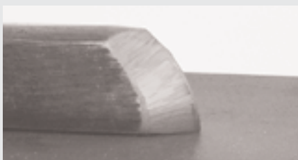
Skews have four surfaces to hone: two ground bevels and two side edges that define the short and long points (shown above).
